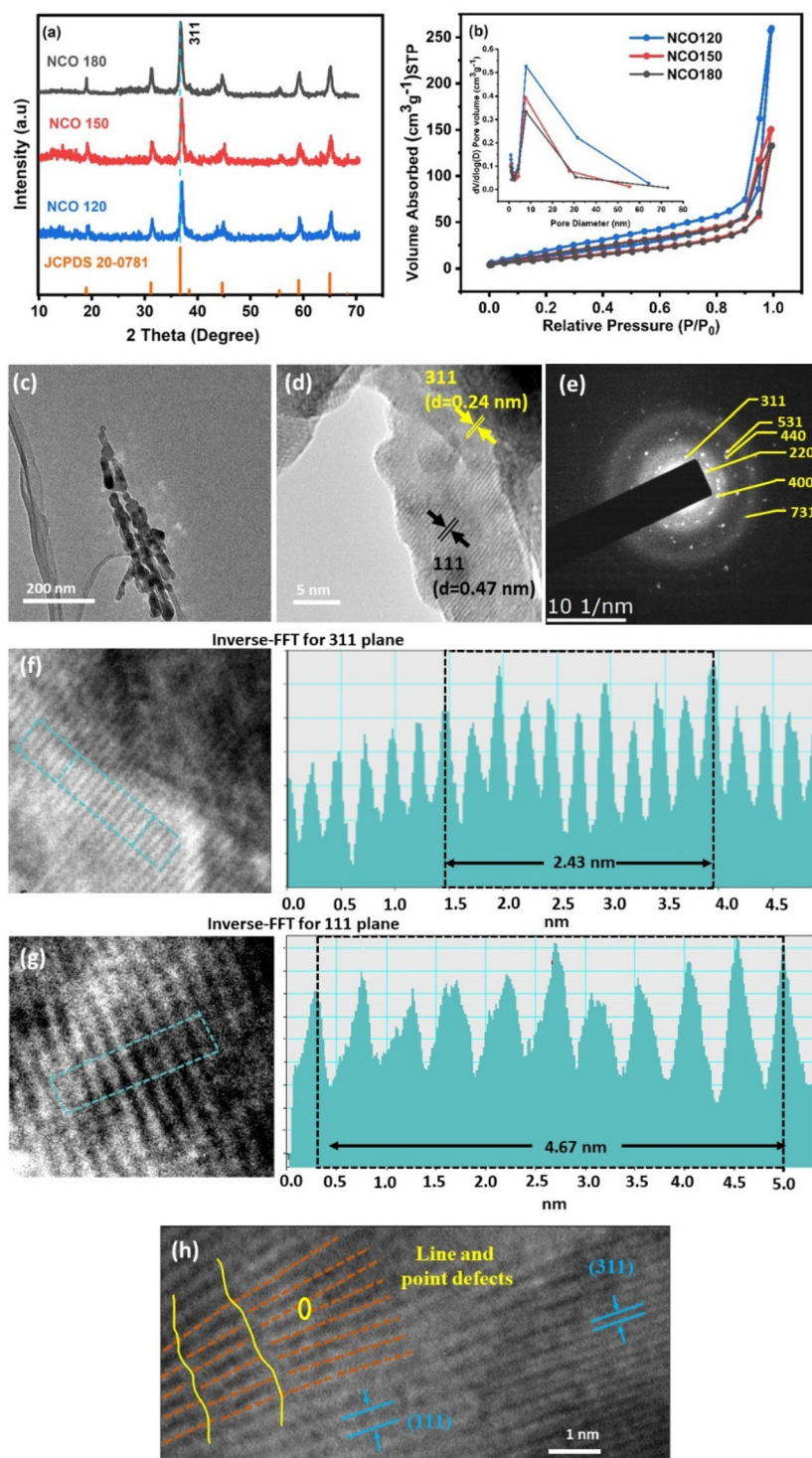
Fig. 2 (a) XRD patterns of the synthesized NiCo 2 O 4 structures on Ni foam, (b) nitrogen adsorption/desorption isotherms and pore size distribution curve of NiCo 2 O 4 structures, (c) TEM image, (d) HRTEM image, (e) corresponding SAED pattern, (f and g) inverse-FFT analysis for the NCO 120 structure, and (h) crystal defects.
