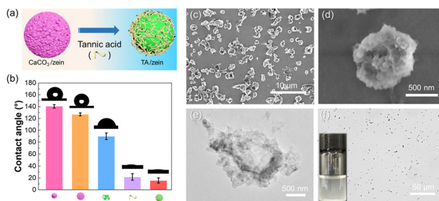
Fig. 3 (a) Schematic representation of the procedure for tannic acid (TA) treatment. (b) The water contact angle of the hydrophobic \text{CaCO}_3 nanoparticles, the \text{CaCO}_3 /zein microparticles, zein powder, tannic acid powder, and TA/zein microparticles. SEM images (c), (d) and TEM image (e) of the TA/zein microparticles. (f) Picture and optical microscopy image of the water-dispersed TA/zein microparticles.
