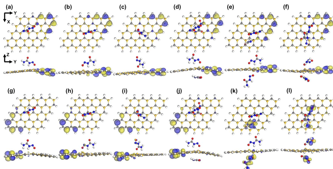
Fig. 3 Top and side views of HOMO ((a)–(f)) and LUMO ((g)–(l)) maps (isovalue = 0.3 a.u.) for S1–S6 configurations of SiC/NU complexes, respectively.
