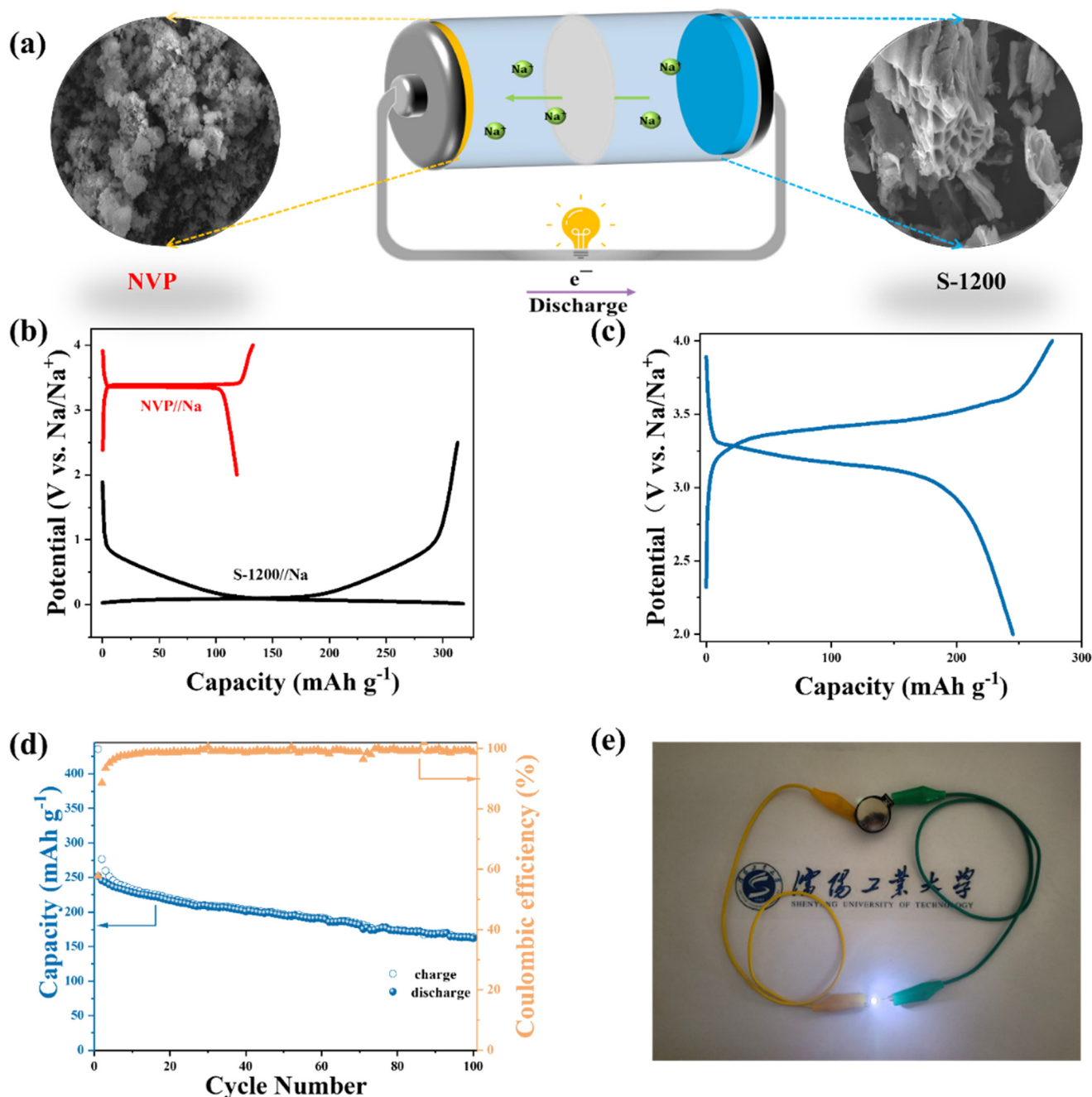
Fig. 5 Electrochemical performance of the full cell: (a) the schematic illustration of the full cell; (b) the galvanostatic charge–discharge curves of NVP//Na and S-1200//Na at 100 mA g -1 ; (c) the galvanostatic charge–discharge curve at 100 mA g -1 ; (d) the cycling stability at 100 mA g -1 ; (e) the optical photograph of a white LED lit by the full cell.
