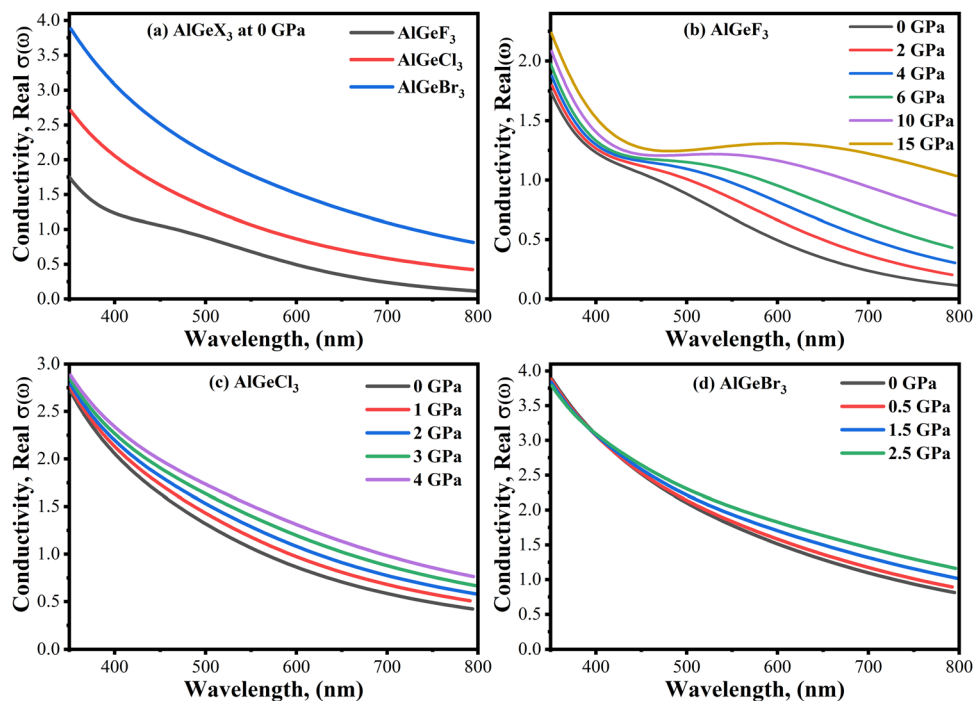
Fig. 11 Comparison of conductivity in visible wavelength range without pressure (a) \text{AlGeX}_3 ( X = \text{F}, \text{Cl}, \text{and Br} ) and with pressure (b) \text{AlGeF}_3 , (c) \text{AlGeCl}_3 , and (d) \text{AlGeBr}_3 .
