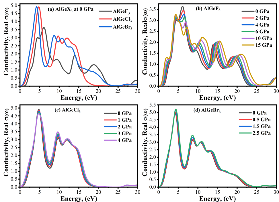
Fig. 10 Comparison of the real part of the conductivity without pressure (a) \text{AlGeX}_3 ( X = \text{F}, \text{Cl}, \text{and Br} ) and with pressure (b) \text{AlGeF}_3 , (c) \text{AlGeCl}_3 , and (d) \text{AlGeBr}_3 .
