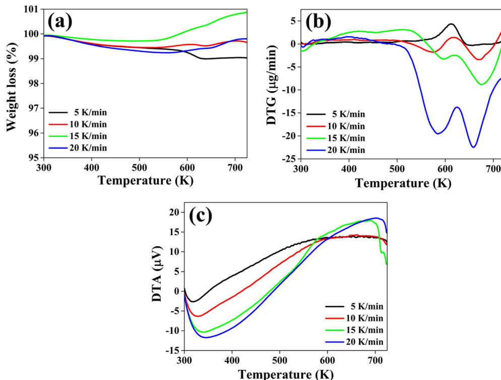
Fig. 14 (a) The TG, (b) DTG, and (c) DTA curves of the grown CuSbSe 2 single crystal.
