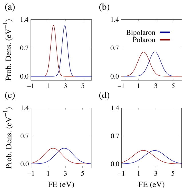
Fig. 5 4AGNR probability density distribution of the polaron (red) and bipolaron (blue) formation energies. (a)–(d) Refer to, respectively, T = 95 , 197, 299, and 350 K cases.
