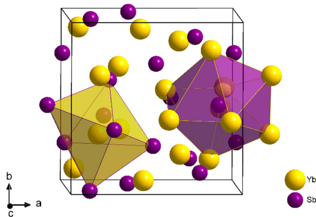
Fig. 1 Crystal structure of \text{Yb}_4\text{Sb}_3 and coordination polyhedra of Yb (yellow) and Sb (purple) atoms.
