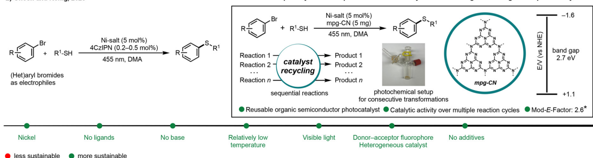
Scheme 1 Representative literature reports on \text{C}(\text{sp}^2)\text{-S} cross-coupling transformations either using palladium or nickel under photoredox dual catalytic conditions with specific ligands and this work. *See ref. 35 and section 5 in the ESI† for more details.
