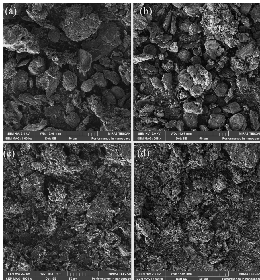
Fig. 1 SEM micrographs of (a) the raw material (black mass leach residue) and the (b) HT-Bat-res, (c) Bat-res-N and (d) HT-Bat-res-BM-N catalyst materials at 1000x magnification.
