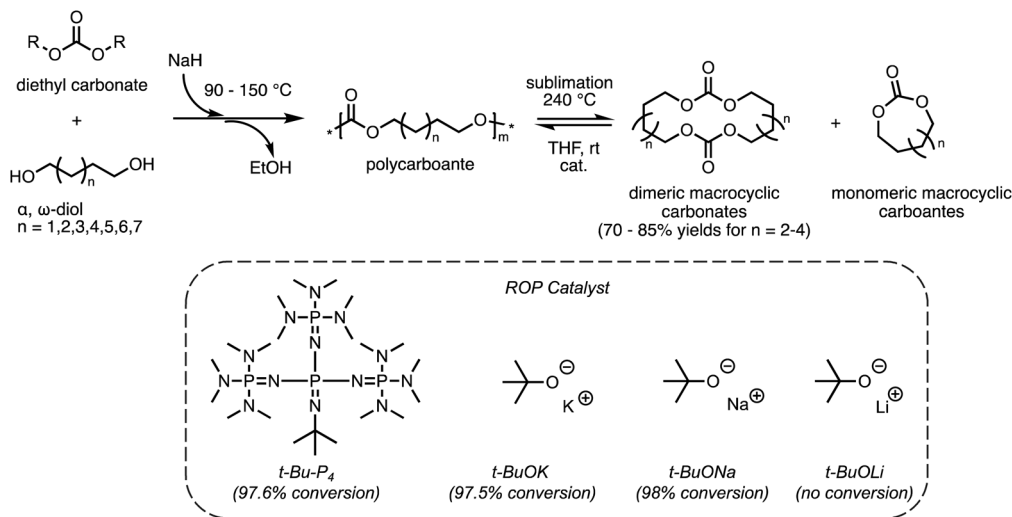
Scheme 4 Polymerization pathway of polycarbonates from \alpha, \omega -diol and diethyl carbonate and its recycling via RCD and ED-ROP. Reproduced from ref. 49 with permission from American Chemical Society, copyright 2022.
