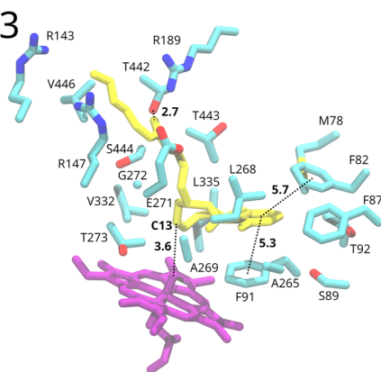
Fig. 3 Protein environment around the substrate in the representative binding poses during the four MD simulations. Distances are shown in Å and represent average distances along the 100 ns of dynamics of poses 2 and 3 and the last 50 ns of dynamics of poses 1 and 4. The substrate is shown in yellow and the heme group in purple. Colours for protein residues: cyan, carbon; red, oxygen; blue, nitrogen; yellow, sulphur.
