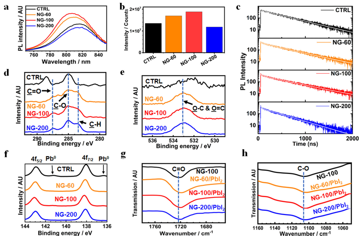
Fig. 5 (a) PL spectra for various perovskite/nanogel systems. (b) The maximum PL intensity from the spectra in (a). (c) TRPL data for various perovskite/nanogel systems. (d) C 1s, (e) O 1s and (f) Pb 4f core level spectra from XPS measurements for the control perovskite and films prepared with nanogels (3 mg g -1 ). (g) C=O and (h) C-O stretching regions of the FTIR spectra measured for NG-100 and the various nanogels mixed with PbI 2 .
