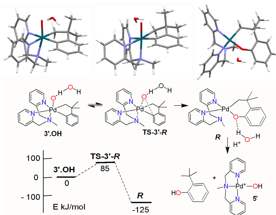
Fig. 8 The calculated structures and relative energies ( E , kJ mol -1 ) for reductive elimination from model complex 3'.OH to give intermediate R . Calculated bond parameters: 3'.OH , Pd–C(Ar) 2.05, Pd–O 2.01, O...C(Ar) 3.00, Pd–N 2.31, Pd–py(t-Ar) 2.20, PdOH–H 1.37, PdOH–O 1.15 Å, O–Pd–C(Ar) 95.0°; TS-3'-R , Pd–C(Ar) 2.14, Pd–O 2.01, O...C(Ar) 2.36, Pd–N 2.36, Pd–py(t-Ar) 2.36, PdO–H 1.40, PdOH–O 1.11 Å, O–Pd–C(Ar) 69.2°; R , Pd...C(Ar) 2.94, Pd–O 2.07, O–C(Ar) 1.38, Pd–N 2.74, Pd–py(t-O) 2.09, PdO–H 1.69, PdOH–O 1.02 Å, O–Pd–C(Ar) 25.3°.
