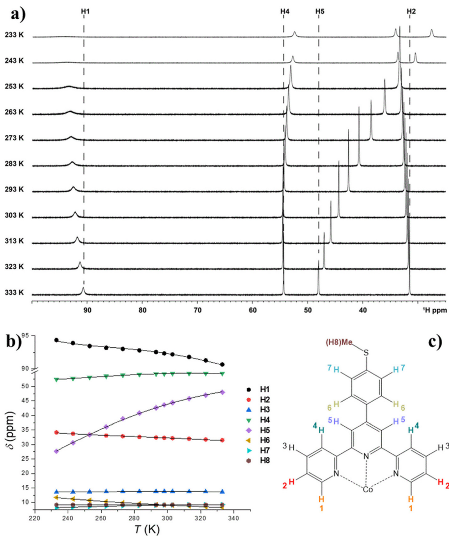
Fig. 6 Panel a: 1 H-NMR spectra of an acetonitrile-d 3 solution of 1 acquired at different temperatures (dashed lines indicates the chemical shifts assignment). Only selected resonances are shown for clarity. Panel b: Temperature dependence of the chemical shifts of every non-equivalent hydrogen of 1 . Lines are the best fitting curves, whose function and parameters are described in the text. Panel c: 1 H assignments for the TerpyPhSMe ligand in 1 .
