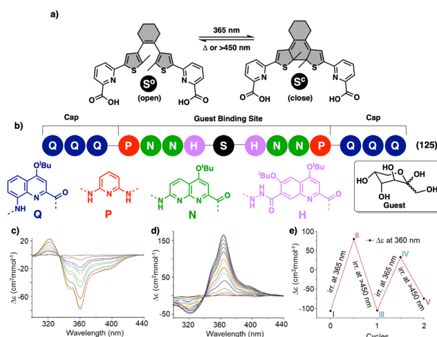
Fig. 59 (a) Structure of DAE core and (b) oligoamide sequence of 125 . CD spectra showing an increase of chirality after irradiation with different wavelengths: (c) \lambda = 365 nm and (d) \lambda = 450 nm. (e) CD switching upon subsequent irradiation cycles. Reproduced from ref. 294 with permission from the Royal Society of Chemistry, copyright 2021.
