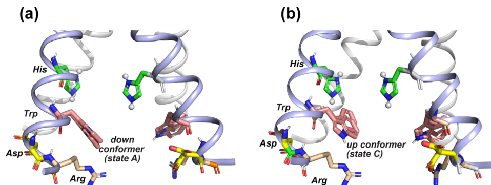
Fig. 8 Provisional model of the tryptophan sidechain conformation that regulates the interactions of this residue with the N-terminal proton-selective histidine and the C-terminal charged residues. The crystal structure of AM2 at pH 5.5 (PDB: 4QKM) is used for modeling. 29 Key residues (H37, W41, D44 and R45) in two neighboring chains (light blue) are shown as sticks. H37 is cationic in this crystal structure. (a) A putative tryptophan down conformer (state A) that interacts with the C-terminal charged residues. The Trp ( \chi_1, \chi_2 ) torsion angles in the left chain are slightly modified to ( -175^\circ, -75^\circ ) from the original structure. The original structure has Trp ( \chi_1, \chi_2 ) torsion angles of ( -175^\circ, -90^\circ ), which are shown in the chain on the right. (b) A putative tryptophan up conformer (state C) that interacts with the cationic histidine. The Trp ( \chi_1, \chi_2 ) torsion angles in the left chain are modified to ( -155^\circ, +135^\circ ) from the original structure to depict this state.
