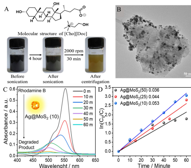
Fig. 14 (A) Molecular structure of [Cho][Doc] and exfoliation of MoS_2 in aqueous [Cho][Doc] ; (B) TEM image showing Ag NPs adhered to the MoS_2 ; (C) time-dependent UV absorbance of RhB in the presence of Ag@MoS_2(10) under sunlight; and (D) comparison of the kinetics of Ag@MoS_2(10) NCs, Ag@MoS_2(25) NCs and Ag@MoS_2(50) NCs. Adopted from ref. 161 with permission. Copyright 2024 Elsevier B.V.
