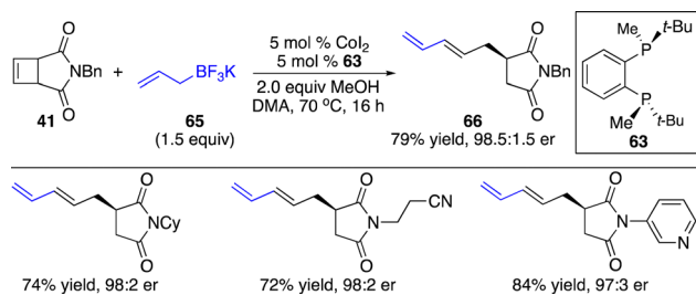
Scheme 22 Co-catalyzed enantioselective cascade allyl addition to cyclobutenes.
