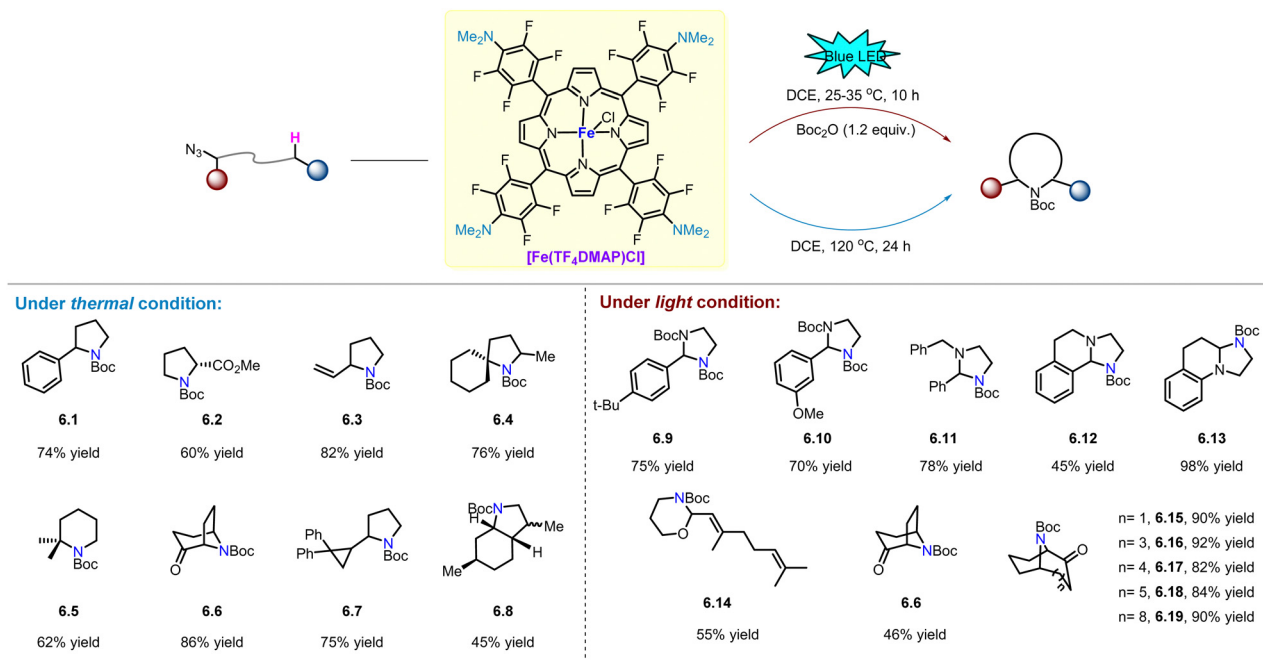
Scheme 6 [Fe III (TF 4 DMAP)OTf]-catalysed intramolecular C(sp 3 )-H amination of alkyl azides under light and thermal conditions.
