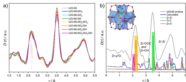
Fig. 2 (a) PDF of the MOFs in the 1.0–5.5 Å range showing peaks centered at 2.2 and 3.5 Å typical from Zr–O and Zr···Zr correlations, respectively. (b) Comparison of the experimental D(r) of the pristine UiO-66 with the calculated partial g(r) s using PDFGUI (ADP values are approached to 0.0005). Main correlations are highlighted in pink, yellow and green.
