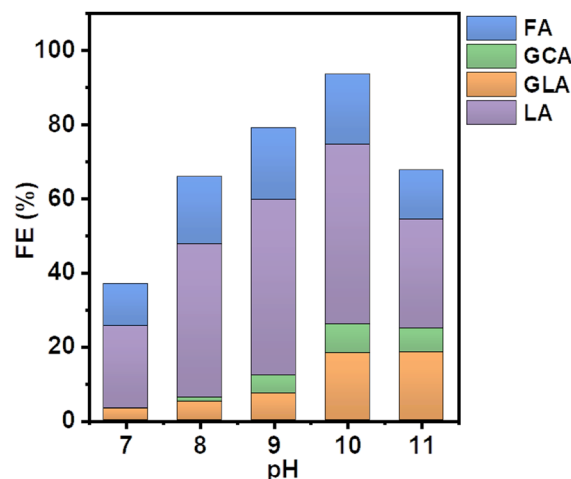
Fig. 3 Faraday efficiencies (FE) of the EGOR at a constant current density of 5 mA cm -2 at various pH conditions in the presence of borate.
