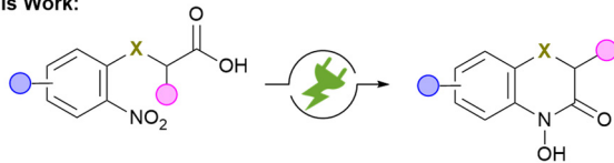
Scheme 2 Conventional and electrochemical reduction of nitroarenes for the synthesis of 2H,4H-4-hydroxy-1,4-benzoxazin-3-ones; C gr = graphite.
