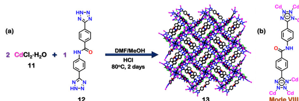
Fig. 5 (a) Schematic representation for the formation of 13 . Crystal structure of 13 was obtained from ref. 87 [color code: blue, N; black, C; magenta, Cd; red, O; green, Cl (H atoms and anions omitted for clarity)]. (b) Binding mode of ligand 12 .
