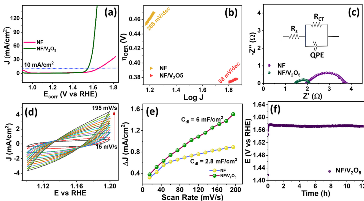
Fig. 3 Electrochemical studies of Ni foam and Ni/ \text{V}_2\text{O}_5 nanorods: (a) LSV profile and (b) Tafel plots, (c) Nyquist plots (inset: cell equivalent circuit), (d) CV plots of \text{Ni}/\text{V}_2\text{O}_5 at different scan rates, (e) EDLC plots to determine C_{dl} and (f) stability analysis of \text{NF}/\text{V}_2\text{O}_5 using chronopotentiometry.
