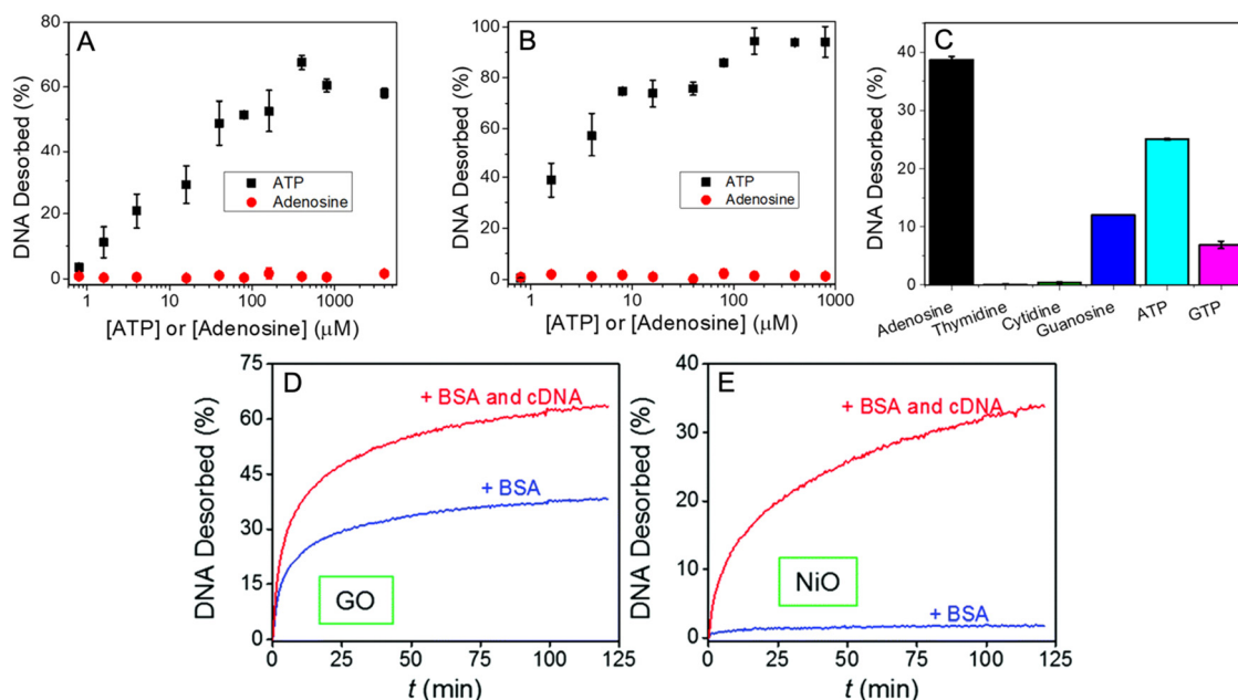
Fig. 4 Concentration-dependent response of fluorescently-labeled-aptamer-coated \text{CeO}_2 NPs upon addition of ATP and Ade using the (A) Ade/ATP aptamer or (B) \text{A}_{15} oligonucleotide. (C) Fluorescent response using fluorescently-labeled aptamer on a GO surface with the addition of various target analytes. Adapted from ref. 41 with permission from the American Chemical Society. Fluorescent response of desorbed probe DNA induced by BSA or BSA + cDNA using (D) GO and (E) NiO as a function of time. Adapted from ref. 42 with permission from the Royal Society of Chemistry.
