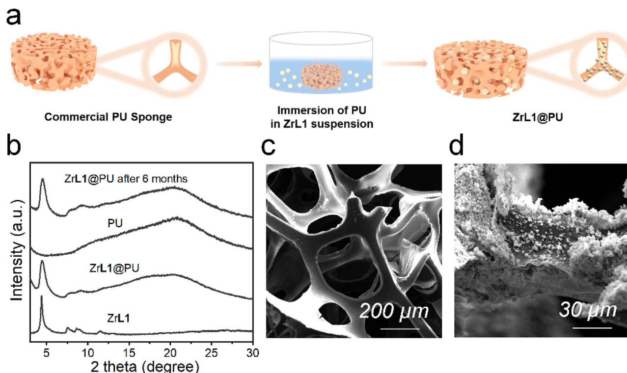
Fig. 2 (a) Schematic depiction of preparation of ZrL1@PU; (b) PXRD patterns (Cu K \alpha , \lambda = 1.5418 Å) of ZrL1 and as made ZrL1@PU, PU, and ZrL1@PU stored for six months; SEM images of (c) PU sponge and (d) ZrL1@PU.
