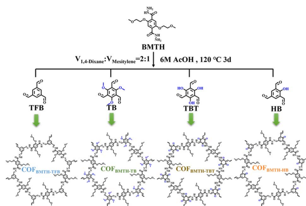
Scheme 1 Synthesis procedures and the structures of COF BMTH-TFB , COF BMTH-TB , COF BMTH-TBT and COF BMTH-HB .
