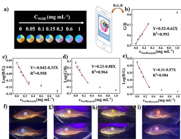
Fig. 5 (a) Photographs of color changes of four aliquots of COF BMTH-TFB , COF BMTH-TB , COF BMTH-TBT and COF BMTH-HB test strips after the addition of 4 \mu\text{L} NOR solution with different concentrations (0, 0.05, 0.1, 0.15, 0.3, 0.6 and 1 \text{mg mL}^{-1} from left to right, respectively). Fitted curves based on (b) COF BMTH-TFB , (c) COF BMTH-TB , (d) COF BMTH-TBT and (e) COF BMTH-HB using a smartphone to detect the NOR concentration via color change. Test paper based on (i) COF BMTH-TFB , (g) COF BMTH-TB , (h) COF BMTH-TBT and (f) COF BMTH-HB to detect fish scales before (top) and after (bottom) the addition of NOR.
