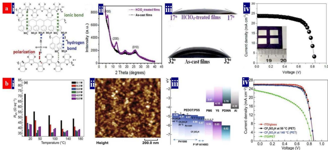
Fig. 2 (a) (i) Inter-molecular interactions among PEDOT, PSS and \text{HClO}_4 ; (ii) XRD spectra of the pristine and \text{HClO}_4 -treated films; (iii) wettability of the droplets (P VP AI 4083) on the pristine and 0.1 M \text{HClO}_4 -treated electrodes; and (iv) J - V characteristics of flexible OSCs with the PEDOT:PSS electrodes (active area: 0.3 \text{ cm}^2 ). Reproduced with permission. 99 Copyright 2020, Royal Society of Chemistry. (b) (i) Sheet resistances of the PEDOT:PSS electrodes; (ii) morphology of PEDOT:PSS nanoparticles; (iii) energy levels of the device components; and (iv) J - V characteristics of flexible OSCs with PEDOT:PSS and ITO electrodes (active area: 0.04 \text{ cm}^2 ), and the rigid OSCs fabricated on ITO/glass substrates. Reproduced with permission. 94 Copyright 2021, Springer Nature.
