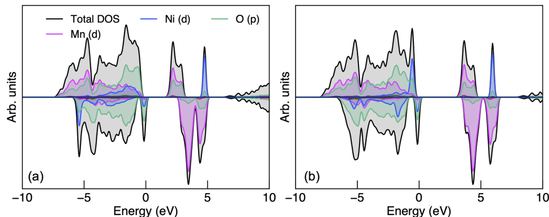
Fig. 2 The electronic density of states of P4_332 \text{LiMn}_{1.5}\text{Ni}_{0.5}\text{O}_4 obtained from (a) PBEsol + U and (b) HSE06 calculations.
