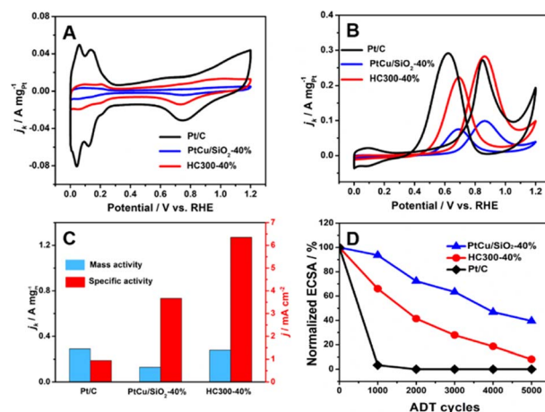
Fig. 4 (A) CVs of commercial Pt/C (20 wt% Pt), PtCu/SiO 2 -40%, and HC300-40%; (B) MOR activity; (C) mass and specific activities obtained from MOR results; (D) accelerating durability tests (ADT) of commercial Pt/C (20 wt% Pt), PtCu/SiO 2 -40%, and HC300-40%.
