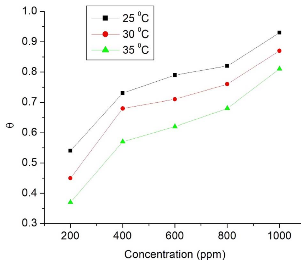
Fig. 11 Henry adsorption isotherm ( \theta ) versus concentration of Co 3 O 4 @PPy NCs at 25, 30, and 35 °C.
