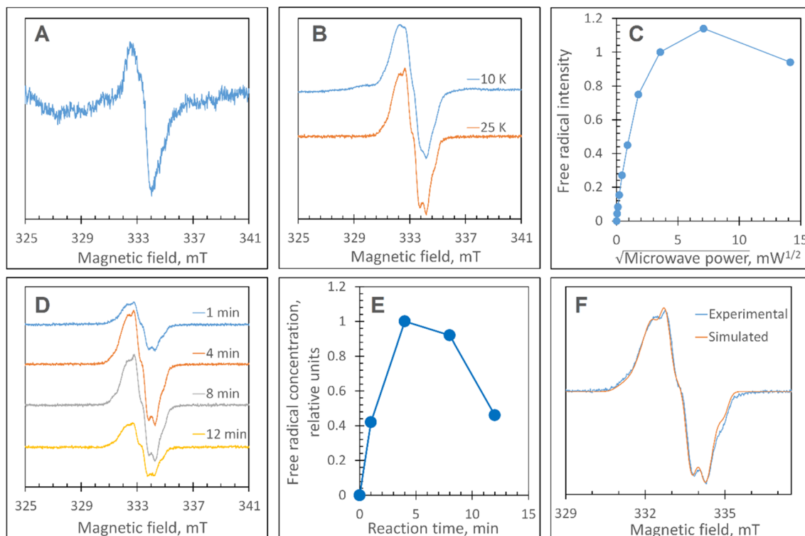
Fig. 6 EPR characterisation of the \text{YO}^\bullet species. (A) The free radical EPR signal detected in the DtpAa double variant, Y345F/F347Y, treated with \text{H}_2\text{O}_2 . The signal is a result of spectra subtraction with variable coefficient and was obtained as follows: 0.26 \times (180 \text{ s}) + 0.68 \times (60 \text{ s}) - 0.47 \times (5 \text{ s}) . In brackets in the formula, are the EPR spectra measured of the samples of 40 \mu\text{M} Y345F/F347Y DtpAa mixed with 400 \mu\text{M} \text{H}_2\text{O}_2 (both concentrations are final – in the mixture) frozen at the times after mixing indicated. (B) The free radical EPR signal formed on the DtpAa triple variant, Y345F/F347Y/Y389F, frozen 6 min after addition of 10-fold excess \text{H}_2\text{O}_2 shows a better line resolution when measured at 25 K as compared to 10 K. (C) The microwave power saturation dependence of the free radical EPR signal (as detected in B). The signal intensities values have been found with the use of the subtraction with variable coefficient. A potentially more accurate procedure of measuring the second integrals of the signals was not easy to implement, as the free radical signal is located on a different EPR signal. (D) The kinetic set of the free radical EPR signals of the 40 \mu\text{M} triple variant DtpAa mixed with 40 \mu\text{M} \text{H}_2\text{O}_2 and frozen various times thereafter (indicated). The spectra have been measured at 25 K whereas the other instrumental conditions were as in A; the spectra have been aligned along the magnetic field to common g values – on the basis of the microwave frequencies used to record each spectrum. (E) The free radical kinetics in relative units as measured from the EPR spectra shown in (D), when using the spectra subtraction with variable coefficient. (F) A TRSSA-Y supported simulation of the free radical EPR signal shown in B (25 K). The TRSSA input parameters were \rho_{\text{C1}} = 0.36 and \theta = 56.5^\circ (or the complementary angle of 61.5^\circ ). The full set of the Hamiltonian parameters generated by TRSSA-Y for this input is reported in Table S1†.
