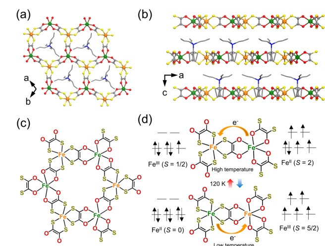
Fig. 10 (a) Two-dimensional honeycomb network of [(n\text{-C}_3\text{H}_7)_4\text{N}][\text{Fe}^{\text{III}}\text{Fe}^{\text{II}}(\text{dto})_3] ( \text{dto} = 1,2\text{-dithiooxalate} = \text{C}_2\text{O}_2\text{S}_2 ). 63 (b) Projection view of the a - c plane: C, gray; O, red; S, yellow; N, blue; Fe III , green; Fe II , orange. 63 (c) Chemical structure of the honeycomb network of (n\text{-C}_3\text{H}_7)_4\text{N}][\text{Fe}^{\text{III}}\text{Fe}^{\text{II}}(\text{dto})_3] . 64 (d) Schematic illustration of the charge-transfer phase transition at 120 K. 64
