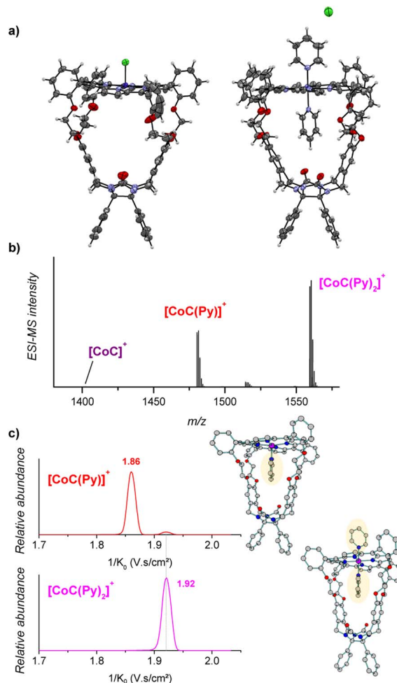
Fig. 2 (a) X-ray structures of [ CoC ](Cl) (left) and [ CoC (Py) 2 ](Cl) (right). Color code: oxygen, red; nitrogen, blue; carbon, gray; hydrogen, white; chloride, green and cobalt, purple. (b) ESI-MS detection of [ CoC ] + ( m/z 1401.4), [ CoC (Py)] + ( m/z 1480.4), [ CoC (Py) 2 ] + ( m/z 1559.4). Additional signals observed at m/z 1515.4 can be attributed to [ CoC – H + Py + Cl] + . (c) Ion mobility separation of [ CoC (Py)] + ( m/z 1480.4 – red mobilogram) and [ CoC (Py) 2 ] + ( m/z 1559.4 – pink mobilogram). DFT-calculated structures of 1 [ CoC (Py IN )] + and 1 [ CoC (Py) 2 ] + , optimized with B3LYP-D3/def2svp, are shown on the right side of the panel.
