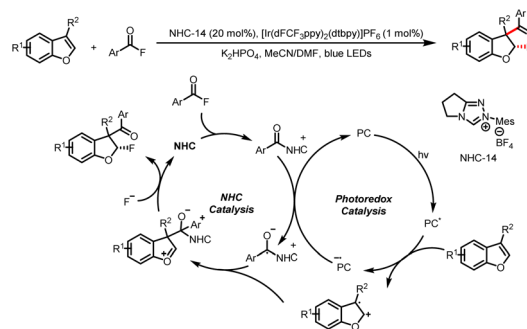
Scheme 35 Construction of 3-aryl-2-fluoro-2,3-dihydrobenzofurans from acyl fluorides and benzofurans.
