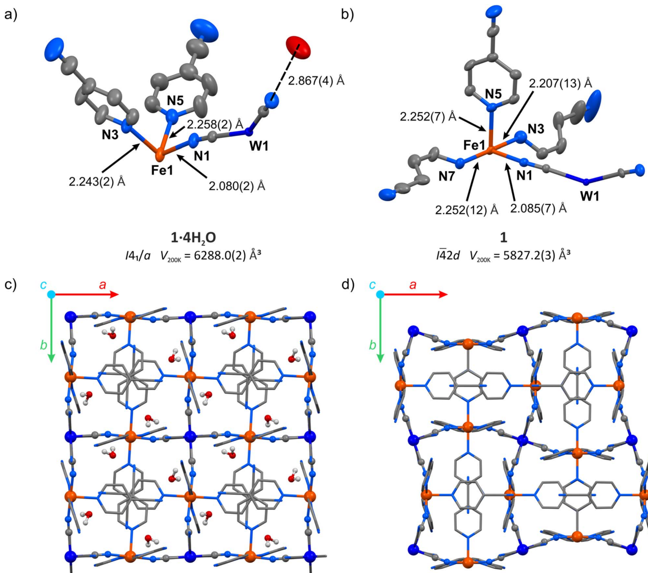
Fig. 2 Structural transformation accompanying the transition from 1 ·4H 2 O to 1 : asymmetric unit of 1 ·4H 2 O (a) and 1 (b) with selected bond distances (hydrogen atoms were omitted for clarity), as well as coordination frameworks of 1 ·4H 2 O (c) and 1 (d) as seen along the crystallographic c -axis (hydrogen atoms of 4-cyanopyridine molecules were omitted for clarity). W – dark blue, Fe – orange, O – red, N – blue, C – grey.
