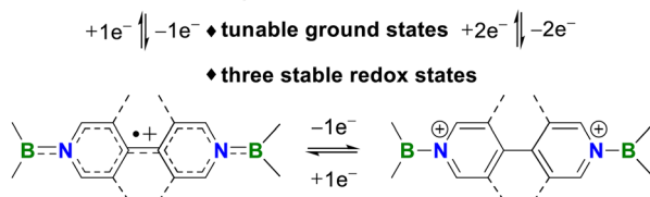
Fig. 1 Resonance forms and redox states of (a) Chichibabin's hydrocarbon and (b) viologens. (c) This work.
