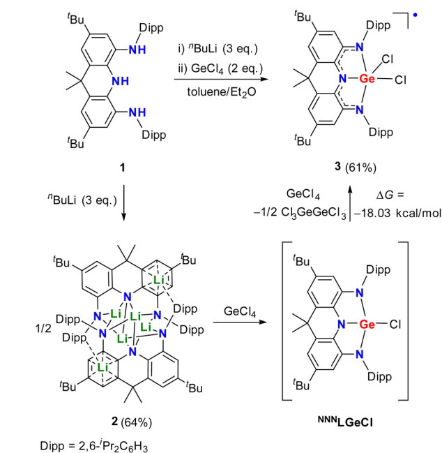
Scheme 1 Synthesis of the germanium precursor 3 .
