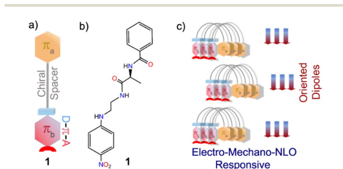
Scheme 1 (a) Schematic representation of molecule 1 with its important structural components: aromatic unit- \pi_a , dipolar unit- \pi_b and the chiral spacer; (b) molecular structure of 1 ; (c) supramolecular assembly of 1 to form highly oriented dipoles to function as an electro-mechano and NLO responsive single-component material.
