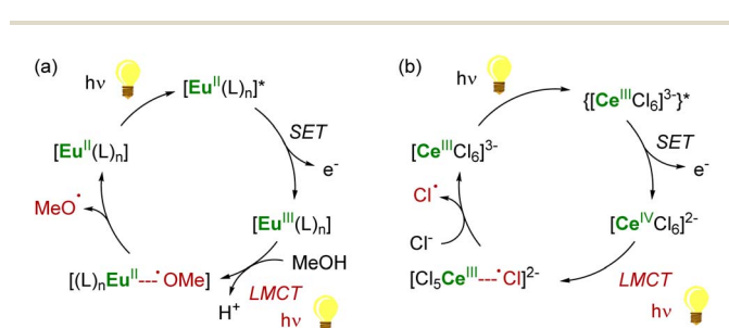
Scheme 7 LMCT-induced homolysis in \text{Eu}^{\text{III}}/\text{Eu}^{\text{II}} (a) 146,149 and \text{Ce}^{\text{IV}}/\text{Ce}^{\text{III}} (photo)catalysis (b). 90
