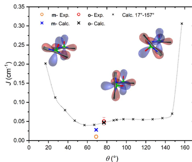
Fig. 4 Magneto-structural correlation of the exchange parameter J ( \text{cm}^{-1} ), vs. \theta ( ^\circ ). The in-plane sp and out-of-plane \pi densities of the two porphyrins are sketched by red and blue lobes, respectively. The black line across the red density indicates the porphyrin planes. Large crosses refer to values computed for the two crystallographic structures, while small crosses refer to simulated geometries obtained varying the tilting angle in o - [\text{VO}(\text{TrPP})]_2 .
