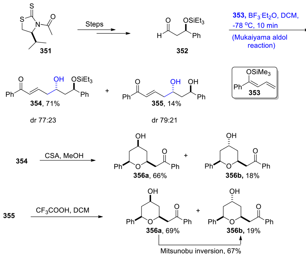
Scheme 47 Synthesis of diospongins 356a and 356b .
