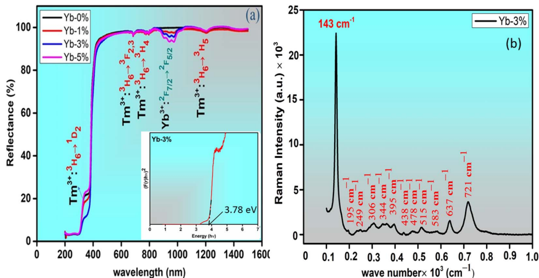
Fig. 4 (a) Diffuse reflectance spectra of (i) Zn_2TiO_4:TM^{3+}-1\%, Yb^{3+}-0\% (ii) Zn_2TiO_4:TM^{3+}-1\%, Yb^{3+}-1\% (iii) Zn_2TiO_4:TM^{3+}-1\%, Yb^{3+}-3\% (iv) Zn_2TiO_4:TM^{3+}-1\%, Yb^{3+}-5\% . The inset shows the optical band gap of the optimized phosphors Zn_{1.96}TiTm_{0.0067}Yb_{0.02}O_4 (Yb-3%) using Kubelka-Munk function (b) Raman spectrum of the optimized sample.
