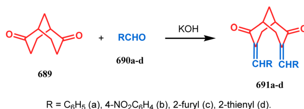
Scheme 156 Synthesis of bicyclo[3.3.1]nonane-based \alpha,\beta -unsaturated diene-dione via aldol condensation.
