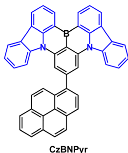
Fig. 40 Molecular structure of CzBNPyr.
