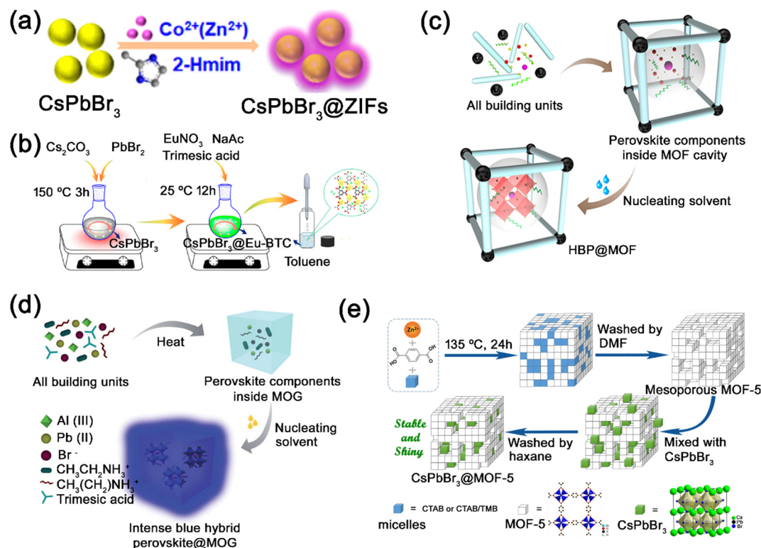
Fig. 14 (a) Schematic illustration of the fabrication process of CsPbBr 3 @ZIF composites. Reproduced from ref. 146 with permission. Copyright 2018, American Chemical Society. (b) Schematic illustration of the external synthesis of CsPbBr 3 @Eu-BTC composites. Reproduced from ref. 133 with permission. Copyright 2019, American Chemical Society. (c) Schematic illustration of the one-pot synthesis of MAPbBr 3 @ZIF-8 composites. Adapted from ref. 134 with permission. Copyright 2019, American Chemical Society. (d) Schematic illustration of the one-pot synthesis of EAPbBr 3 @MOG nanocomposites. Adapted from ref. 147 with permission. Copyright 2019, Royal Society of Chemistry. (e) Schematic illustration of the physical mixing synthesis of CsPbBr 3 @MOF-5 composites. Adapted from ref. 129 with permission. Copyright 2019, Elsevier.
