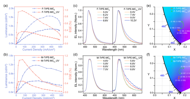
Fig. 4 Device performance of F-TrPE-MC 8 and M-TrPE-MC 8 -based OLEDs. Luminescence–current density characteristics and maximum external quantum efficiency (EQE) versus current density curves for F-TrPE-MC 8 (a), M-TrPE-MC 8 (b)-based OLEDs devices. Electroluminescence (EL) spectra of devices based on F-TrPE-MC 8 (c), M-TrPE-MC 8 (d) pristine film and aged film in the atmosphere, together with their corresponding CIE (e and f), the arrow points into the CIE of increasing current density.
