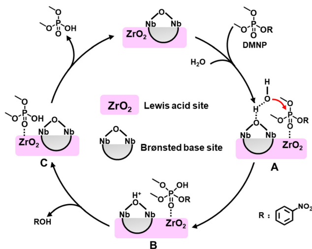
Fig. 7 The possible hydrolytic degradation mechanism for DMNP on the \text{C}_{16}\text{N-Nb}_6/\text{ZrO}_2 catalyst.
