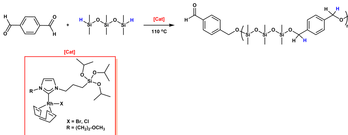
Scheme 8 Hydrostilylation of terephthalaldehyde with hexMTS using \text{Rh}(\text{COD})(2\text{-methoxyethyl-NHC-(CH}_2\text{)}_3\text{Si(OiPr)}_3\text{)Br} homogenous catalyst. Reproduced from ref. 44 with permission from John Wiley and Sons, copyright 2013.
